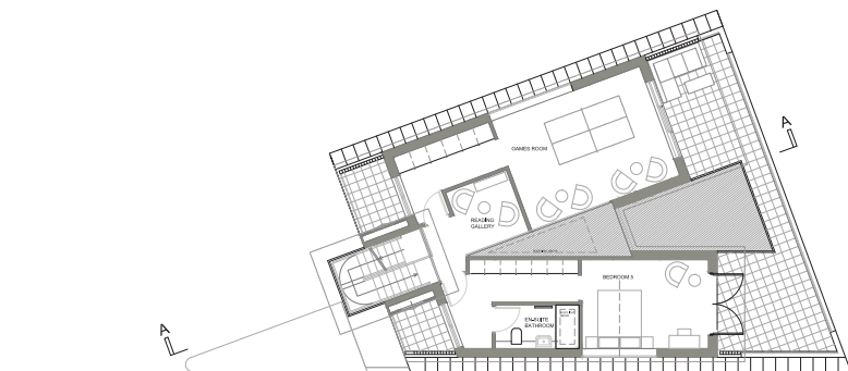
HOUSE A, First Floor Plan (Scale 1:100)
