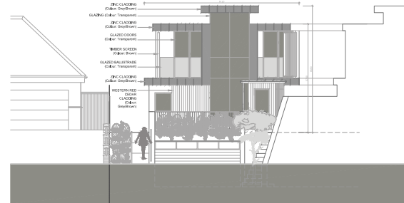
HOUSE A, Southern Elevation (Front) (Scale 1:100)
