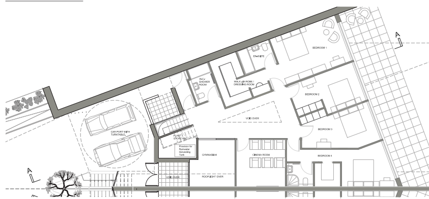
HOUSE A, Lower Ground Floor Plan (Scale 1:100)
