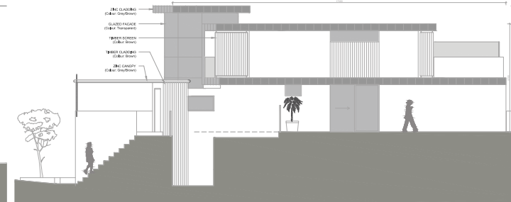
HOUSE A, Eastern Elevation (Side) (Scale 1:100)
