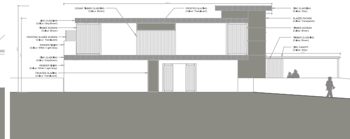
HOUSE A, Western Elevation (Front) (Scale 1:100)
