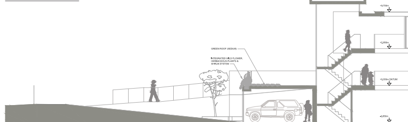
HOUSE A, Section AA (Scale 1:100)
